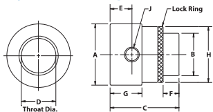
Adjustable Air Amplifier Dimensions
