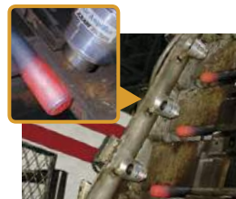
Model 6042 2" (51mm) Adjustable Air Amplifiers with swivel fittings cool inductively heated axles soon after installing the hubs.
